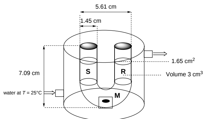
Figure 1. Transport cell, with dimensions.
