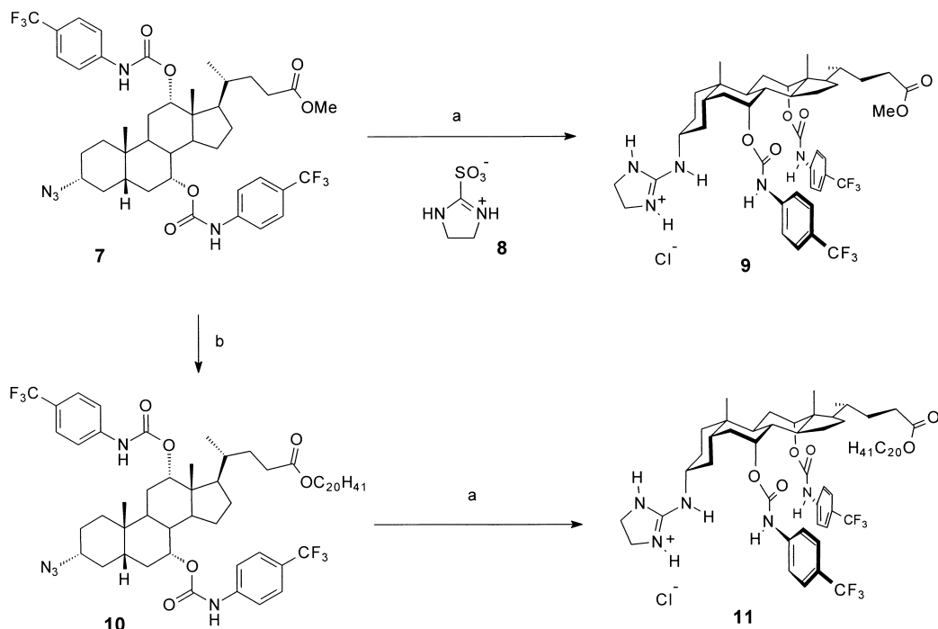
Scheme 1. Synthesis of receptors 9 and 11 : a) 1) Zn, AcOH, 2) 8 , \text{NaHCO}_3 , DMF, 3) \text{CH}_2\text{Cl}_2 , 1M NaOH aq. then 0.5M HCl aq.; b) 1) NaOH, MeOH, \text{H}_2\text{O} , 2) HCl aq., 3) \text{C}_{20}\text{H}_{41}\text{Br} , \text{Cs}_2\text{CO}_3 , NaI (cat.), DMF.
