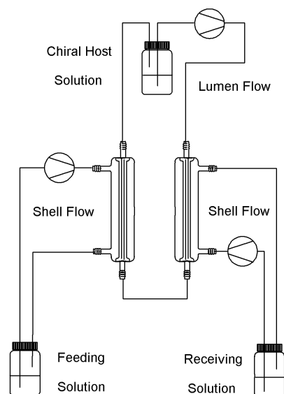
Figure 4. Experimental set-up for simultaneous extraction and stripping of N -Ac-DL-PheOH using two hollow fibre contactors.
