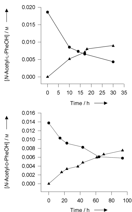
Figure 2. Active transport of N -Ac-PheOH single enantiomers with carrier 11 in U-tube apparatus (Figure 1). Triangles represent receiving phases and circles source phases
